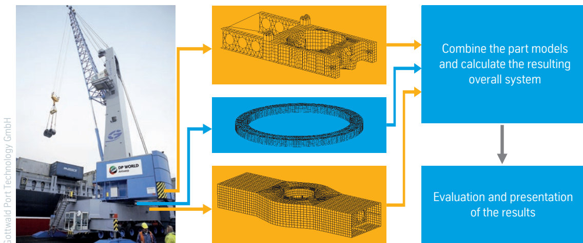
Figure 10: Schematic process
