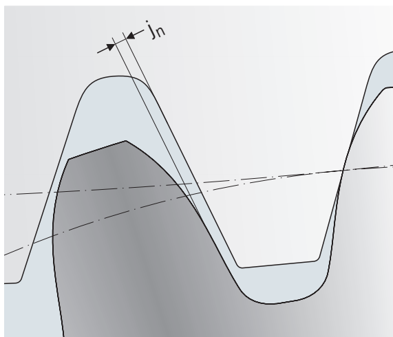
Figure 20: Backlash
