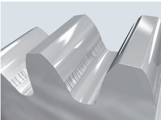
Figure 22: Scuffing
